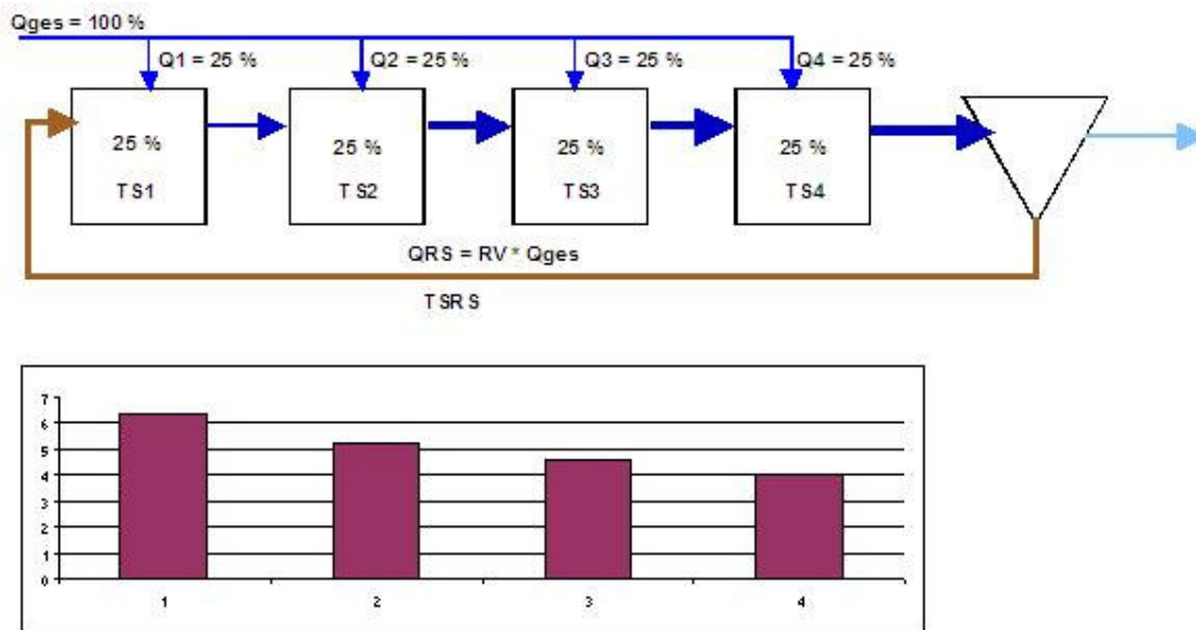
Fig. 45: MLSS for RS = 1 resp. QRS = Qges; "TS" means SS
