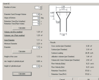
Fig. 121: Screen Circular Chamber
