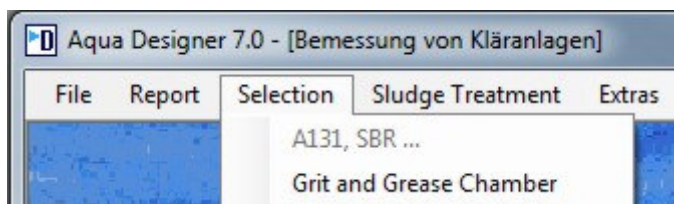
Fig. 118: Menu Selection
