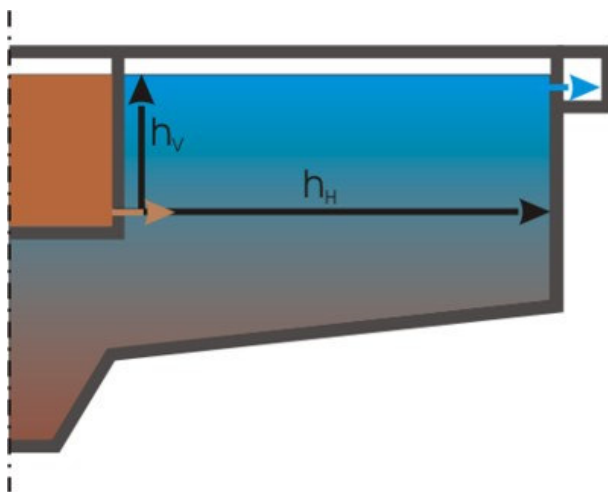
Fig. 83: Flow in the secondary sedimentation
