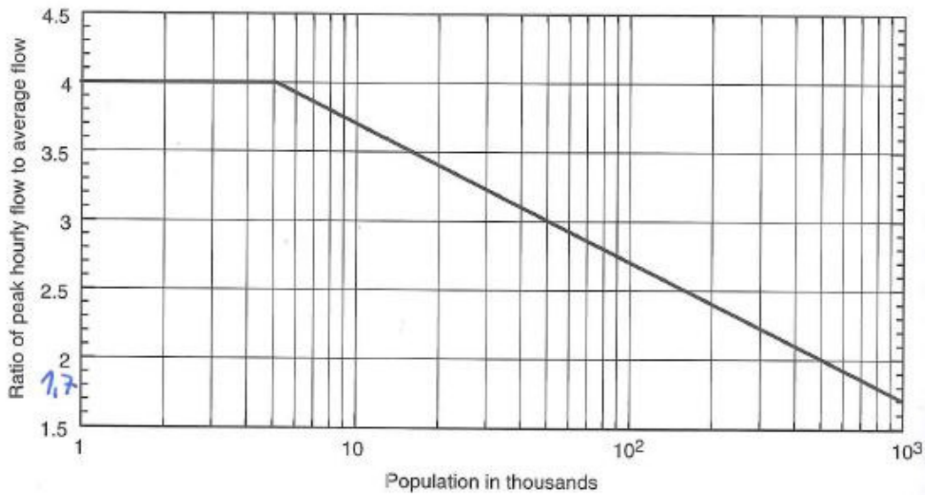
Fig. 36: Peak Factor(Relation of hourly peak to average daily inflow)
