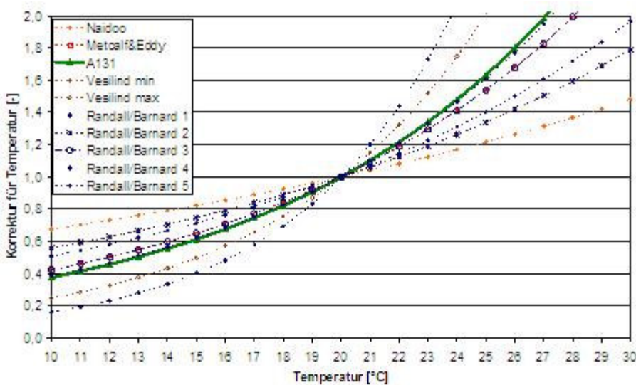
Fig. 51: Correction of temperature
