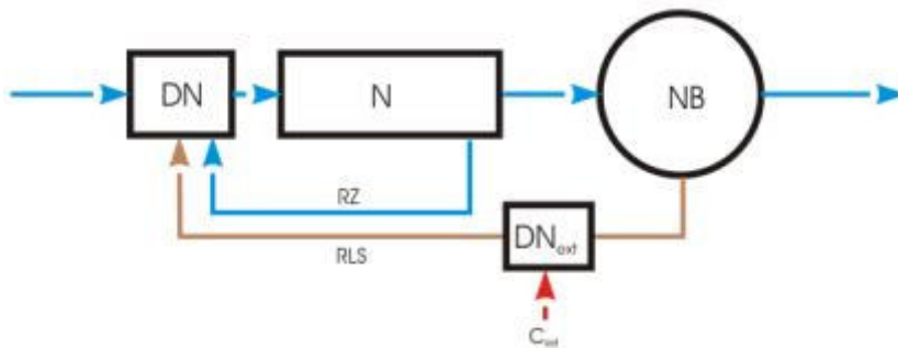
Fig. 49: Only the denitrification of the return sludge with external C
