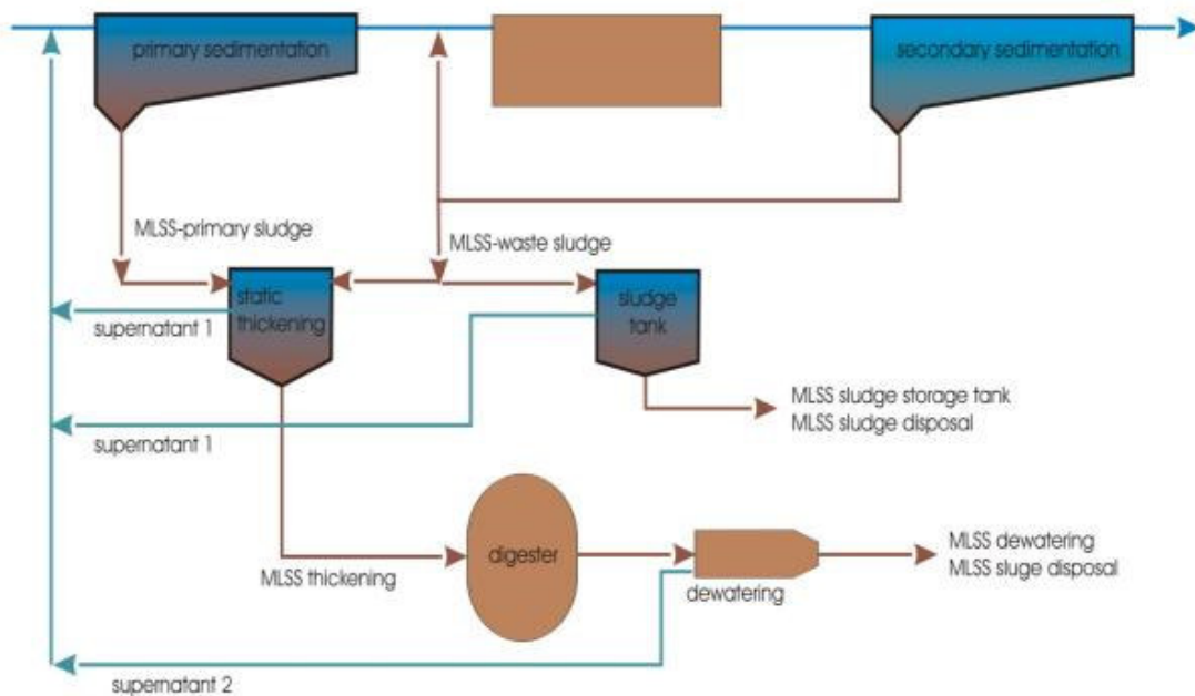
Fig. 39: Flow scheme for supernatant flows
