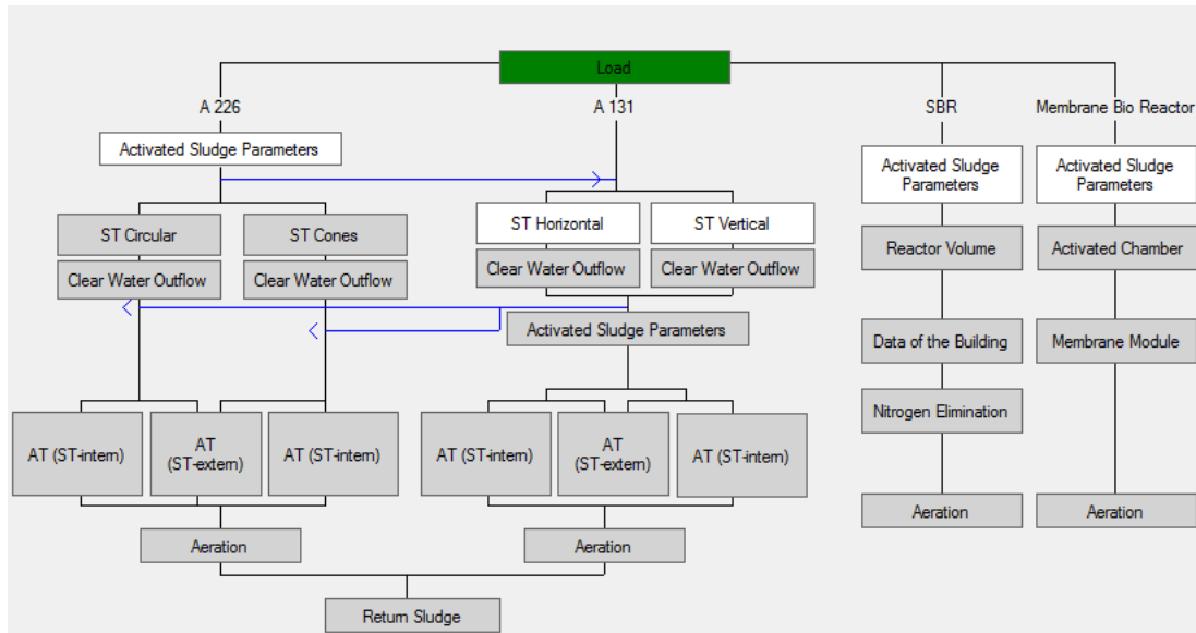
Fig. 41: Main Window for simultaneous aerobic sludge stabilization
