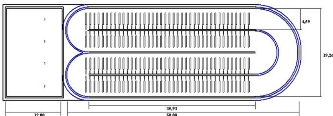
Fig. 105: strip aerators in the nitrification tank
