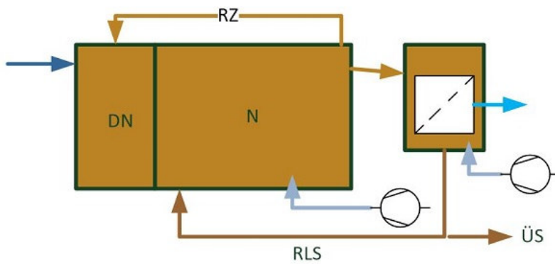
Fig. 109: With external dry installed filtration
