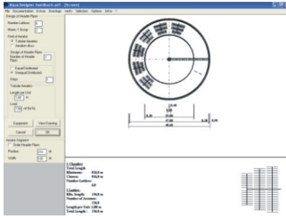
Fig. 157: Combined chamber system, aeration placement
