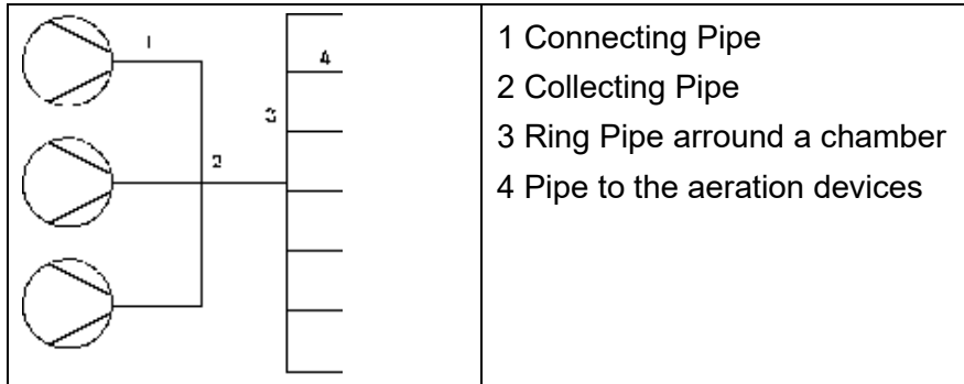
Fig. 143: Air supply pipeline system
