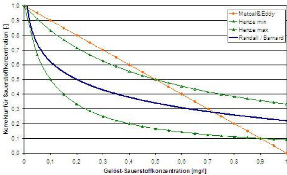
Fig. 50: Correction for the solute oxygen
