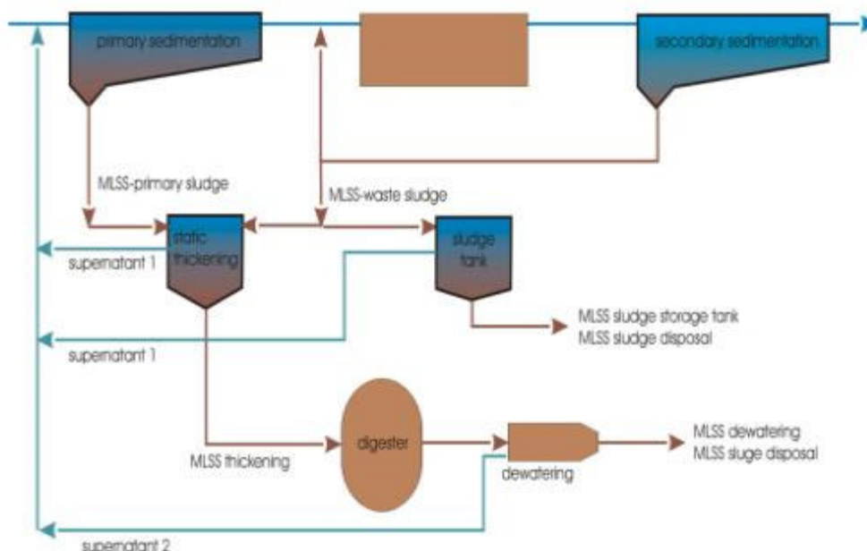
Fig. 180: Steps of Sludge Treatment
