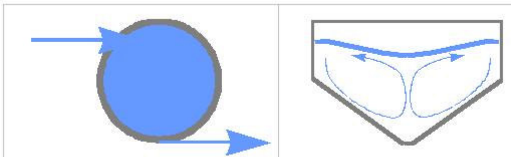
Fig. 120: Stream in Circular Grit Chamber
