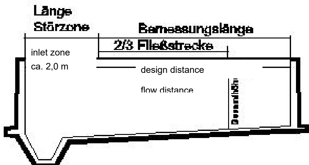
Fig. 76: Rectangular tank measurements (Length of zones)
