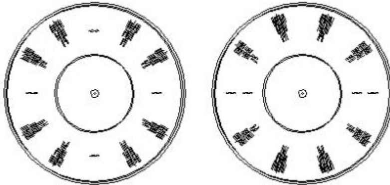
Fig. 101: Selection of mixers per group, one mixer per group in the left example and two mixers per group in the right example
