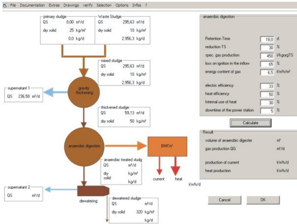
Fig. 137: Form Anaerobic Sludge Digestion
