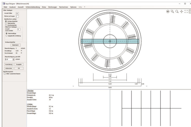
Fig. 21: Membrane Aerator
