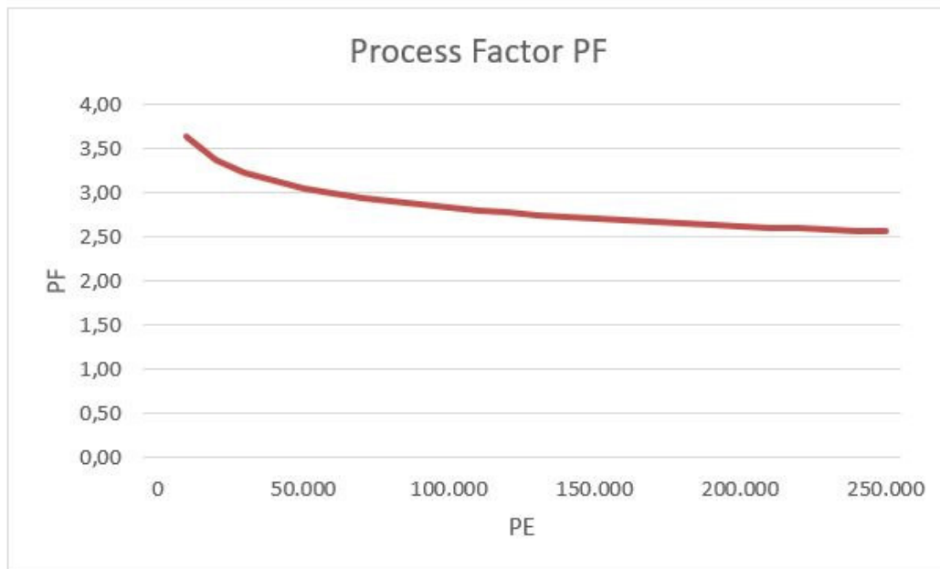
Fig. 37: Process factor MSIG /56/
