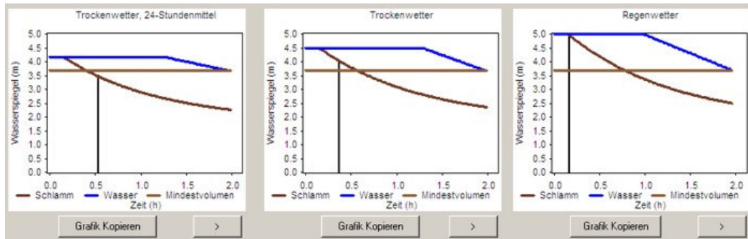
Fig. 115: Proof for dry and rainy weather
