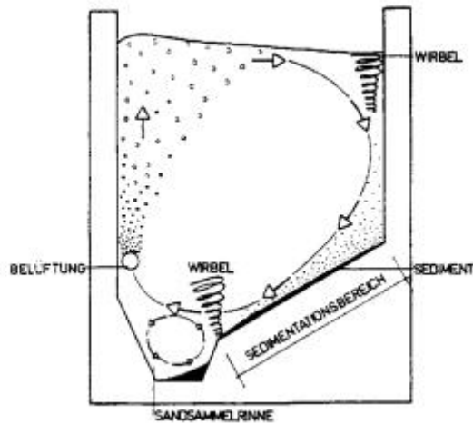
Fig. 122: Cross section of an aerated grit chamber
