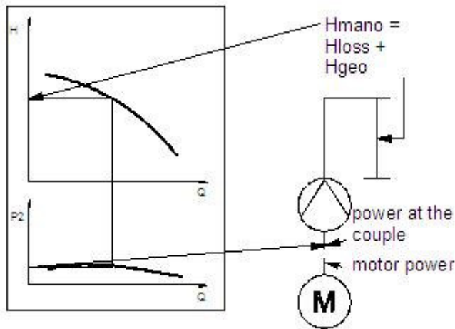
Fig. 130: Pump Characteristics and Capacity
