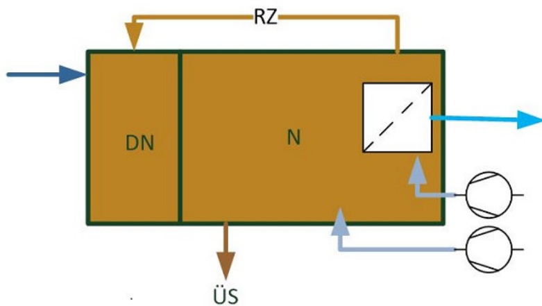
Fig. 111: In the nitrification tank submerged filtration
