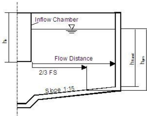
Fig. 79: Horizontal-Flow Secondary Sedimentation Tank
