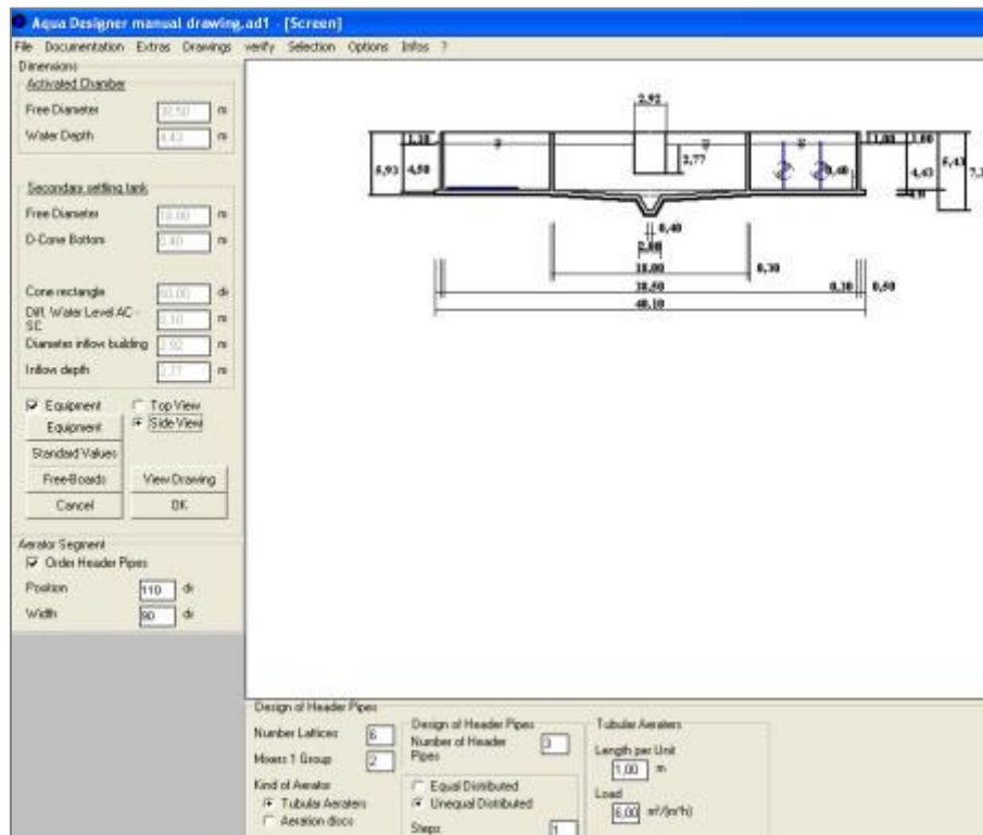
Fig. 148: Form drawings for compact chamber system
