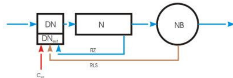
Fig. 47: Integration into the denitrification in a separate basin (DN = Denitrifikation, N = Nitrifikation, NB = ST = sedimentation tank)
