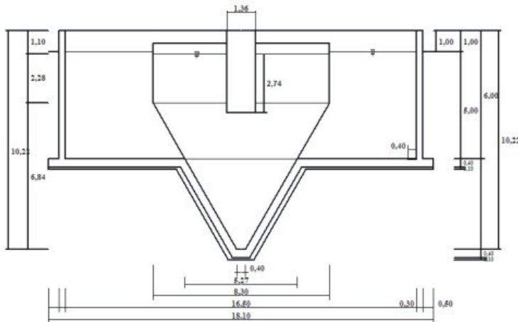
Fig. 93: Scaled Drawing with Measurements
