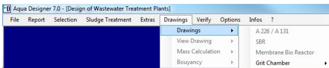
Fig. 145: Menu > Drawings
