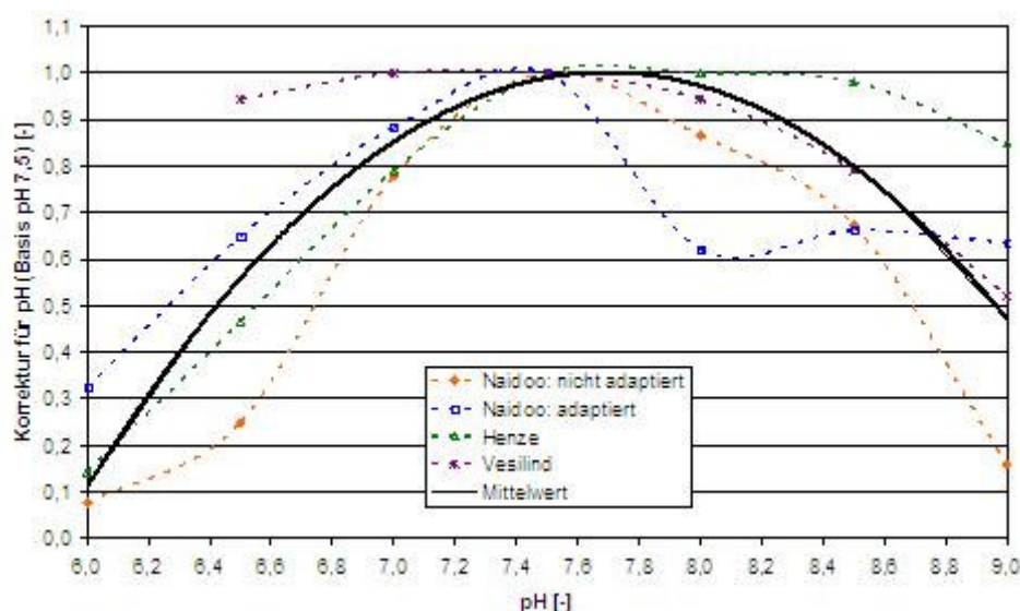
Fig. 52: Correction of pH
