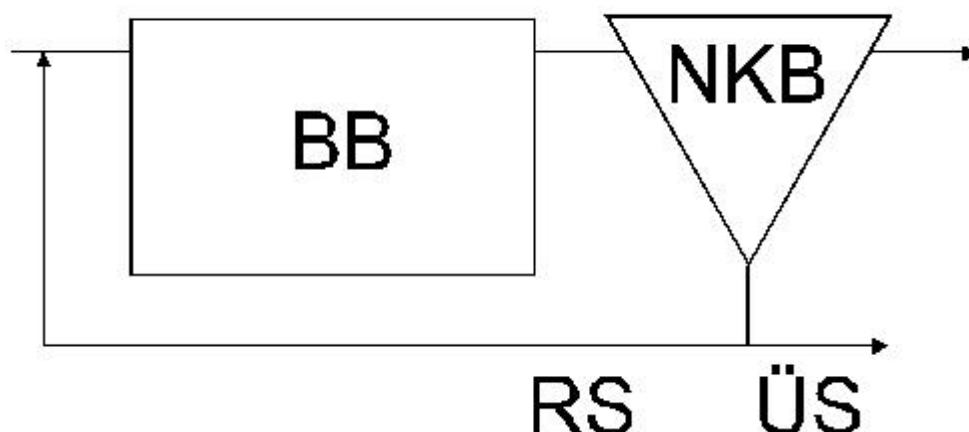
Fig. 28: Activated sludge process (BB = Activated Sludge Tank, NKB = Sec Sedimentation Tank, RS = Sludge Recirculation, ÜS = Excess Sludge)
