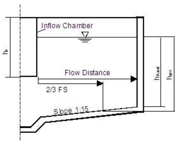
Fig. 77: Horizontal-Flow Secondary Sedimentation Tank
