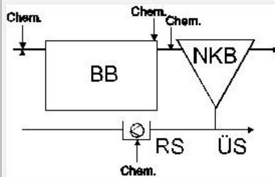
Fig. 59: Possible points of application in the simultaneous precipitation
