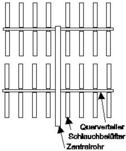
Fig. 103: Aeration lattice with header pipes
