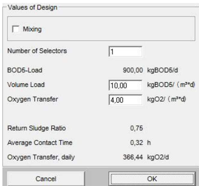
Fig. 69: Options Aerobic Selector
