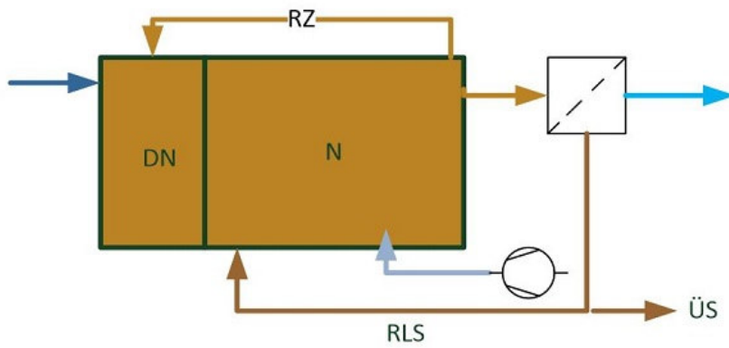
Fig. 109: With external dry installed filtration
