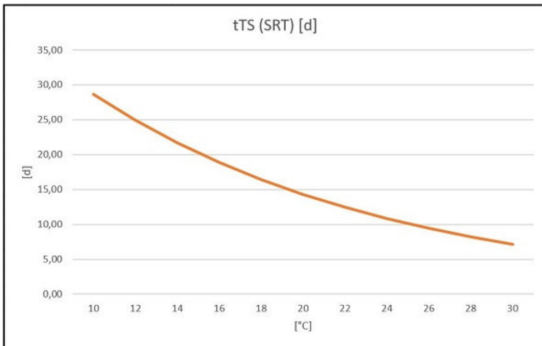
Fig. 55: Temperature dependence of sludge age for simultaneous aerobic sludge stabilization
