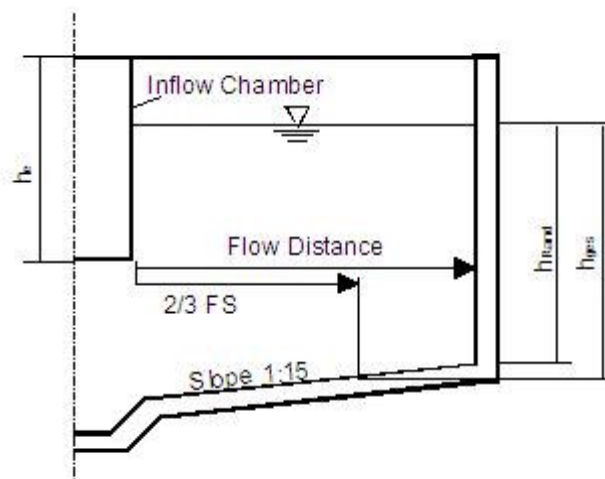
Fig. 73: Design of a secondary sedimentation tank / vertical flow
