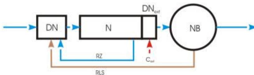
Fig. 48: Integration into the denitrification basin in the downstream stage
