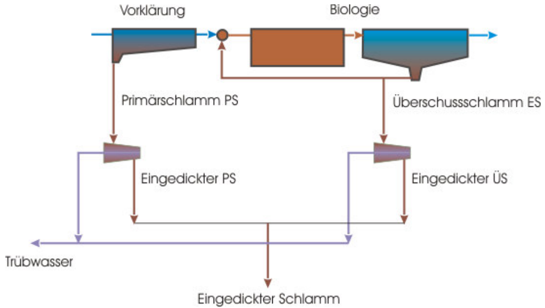
Fig. 139: Sludge thickening
