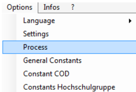
Fig. 42: Options > Process
