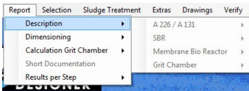
Fig. 133: Menu Report
