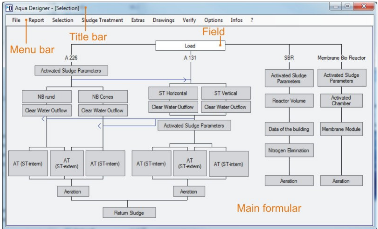
Fig. 3: main window
