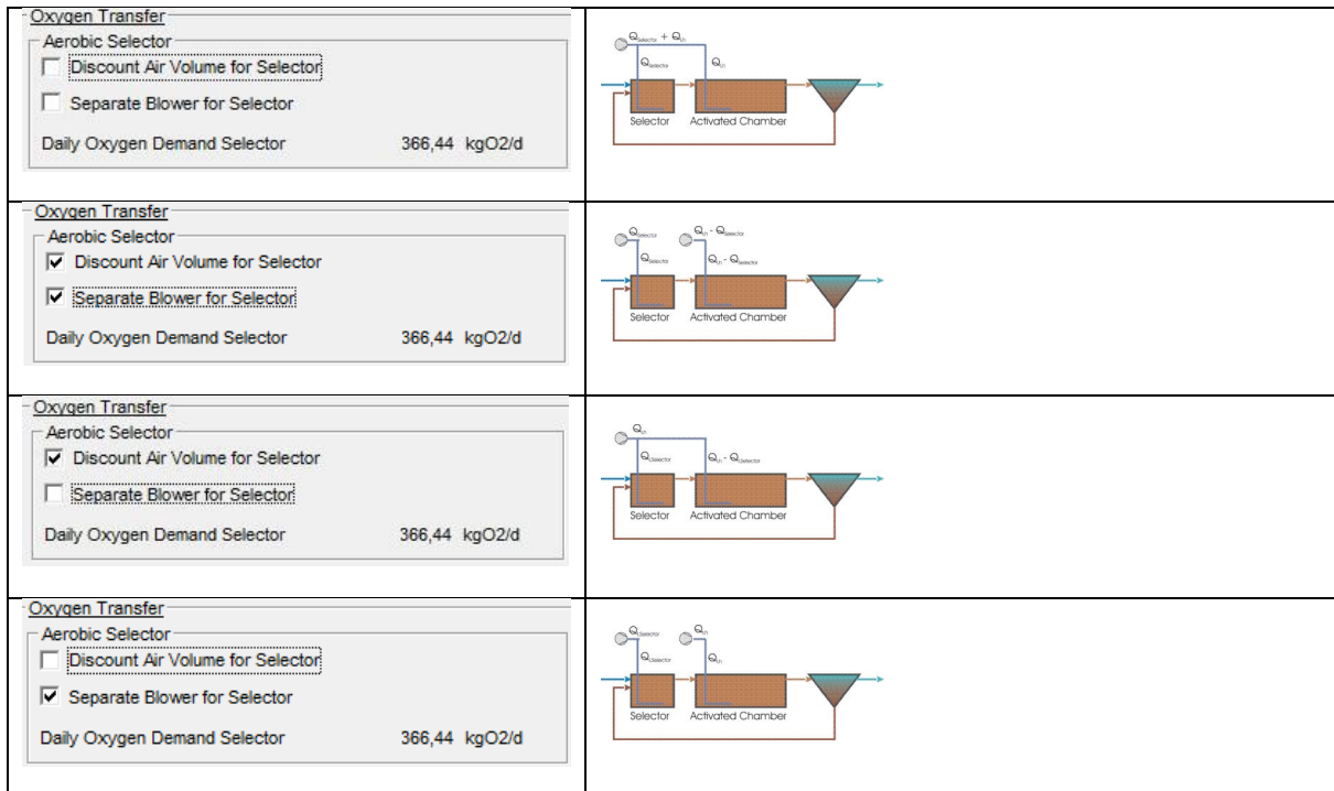
Fig. 68: Variations of the aration of selector and activated chamber
