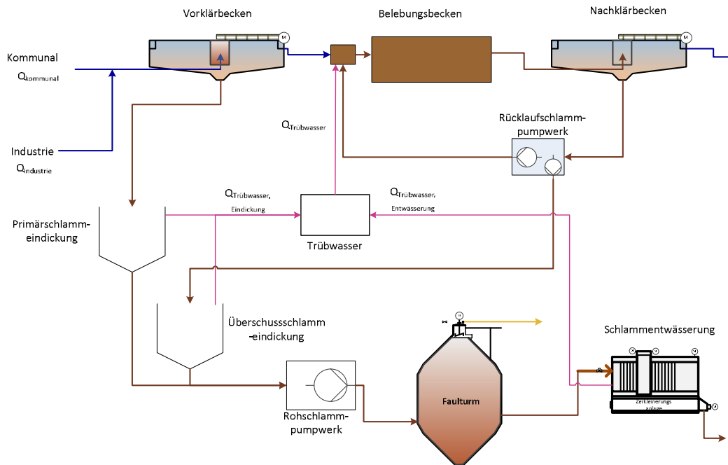
Fig. 40: Material Flows
