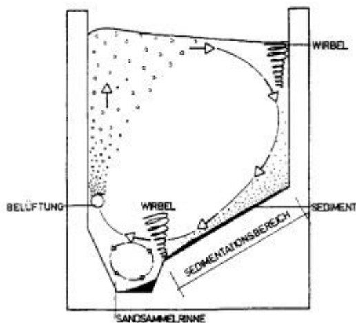
Fig. 114: Cross section of an aerated grit chamber
