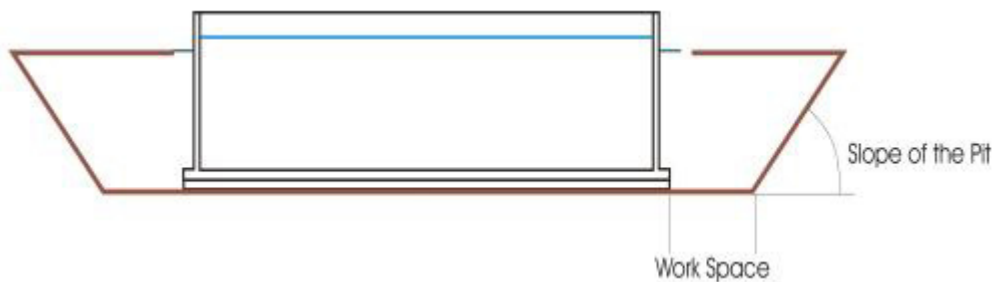
Fig. 144: Pit for activated chamber
