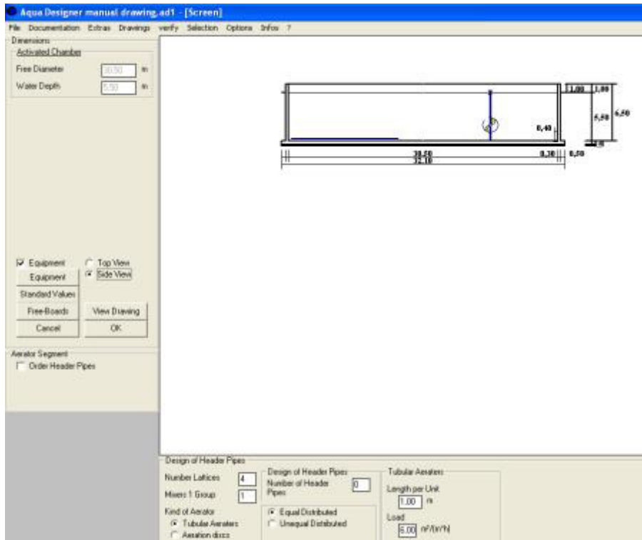
Fig. 136: Form drawings for activated chamber
