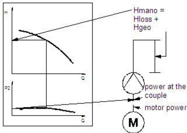
Fig. 121: Pump Characteristics and Capacity
