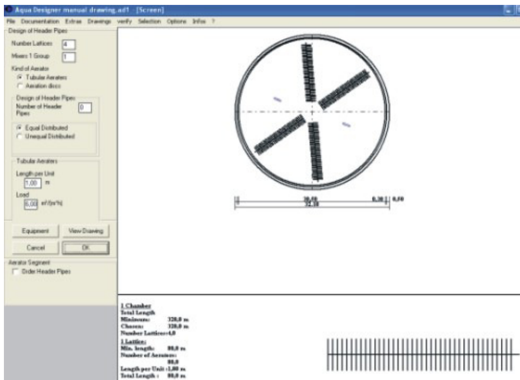
Fig. 140: Activated chamber aeration system
