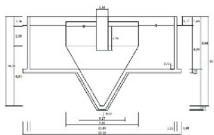
Fig. 91: Scaled Drawing with Measurements
