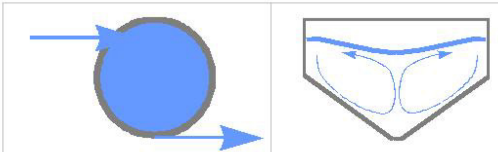
Fig. 112: Stream in Circular Grit Chamber
