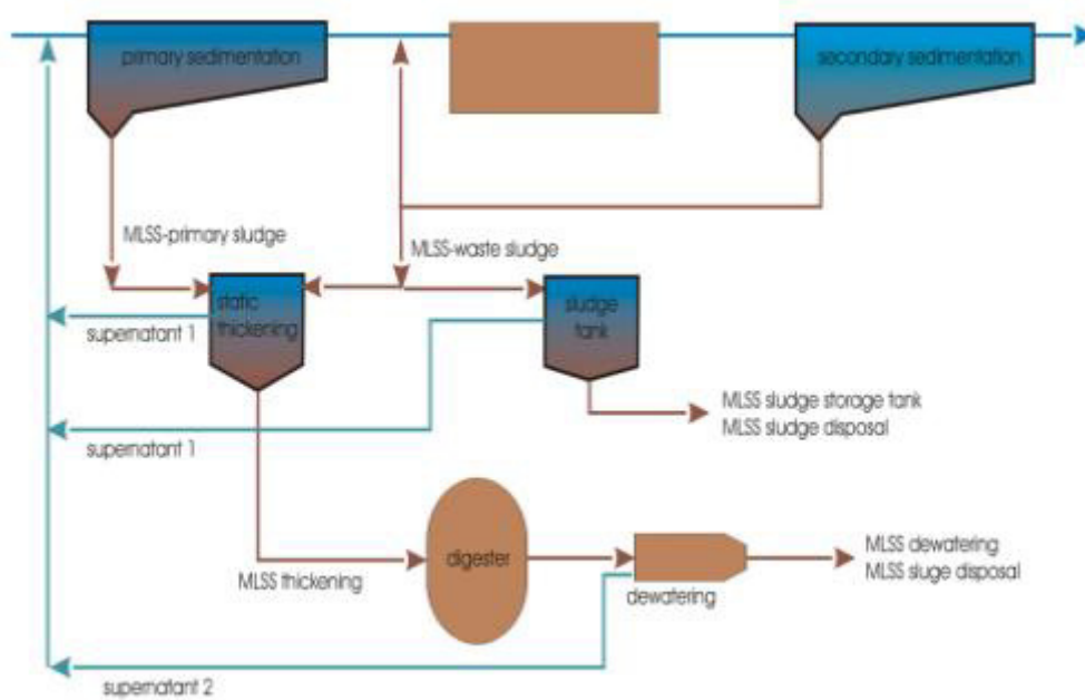
Fig. 163: Steps of Sludge Treatment
