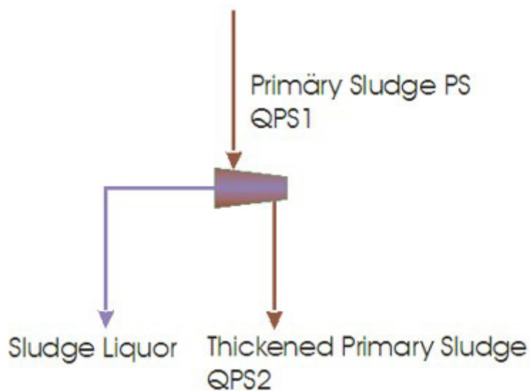
Fig. 130: Material Balances
