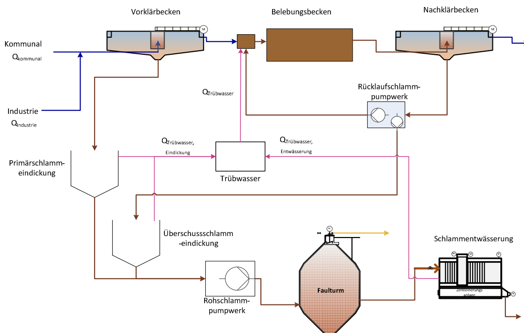
Fig. 38: Material Flows
