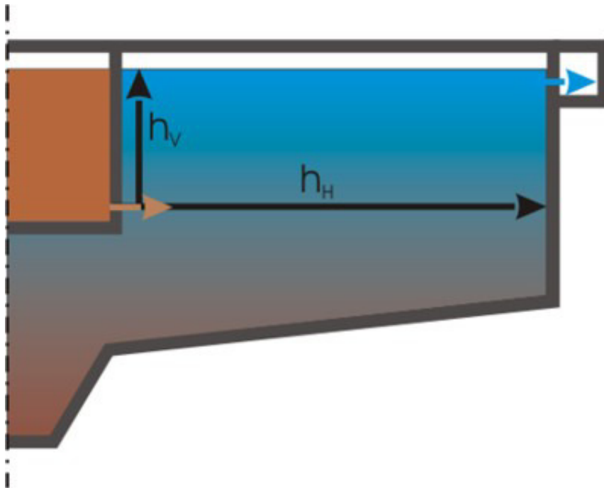
Fig. 81: Flow in the secondary sedimentation
