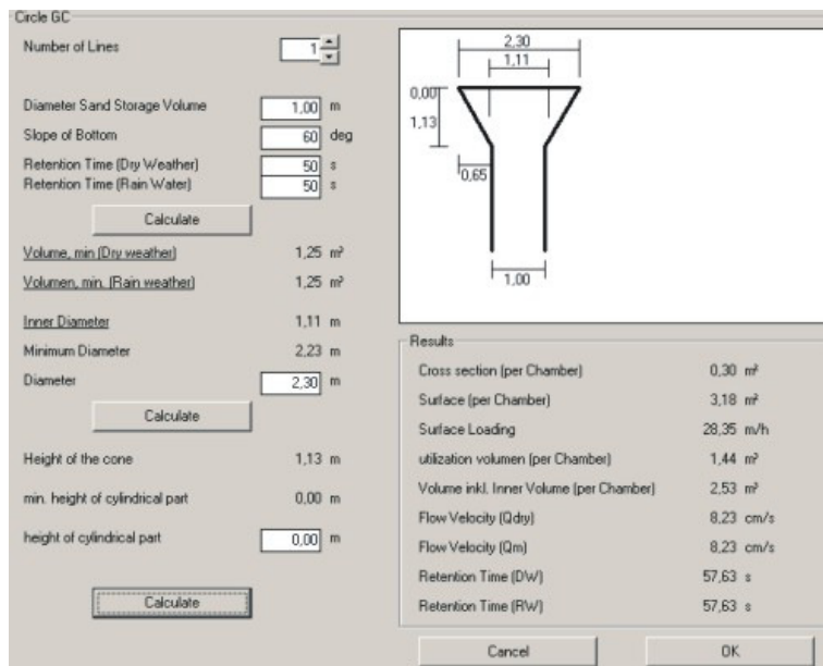
Fig. 113: Screen Circular Chamber
