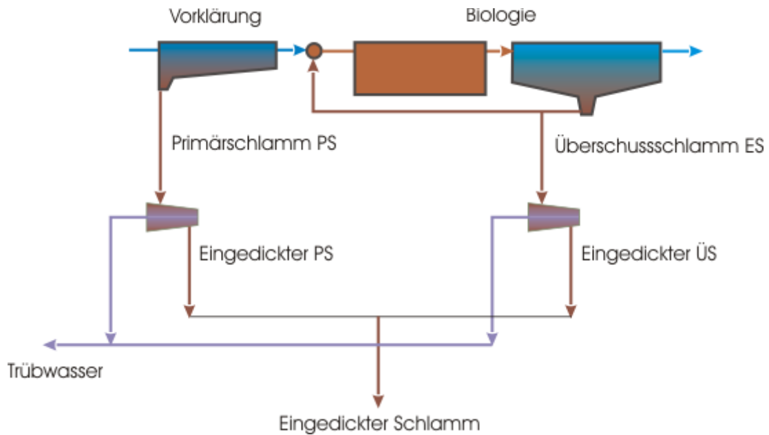
Fig. 129: Sludge thickening
