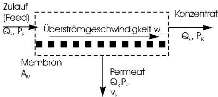
Fig. 106: Membran System
