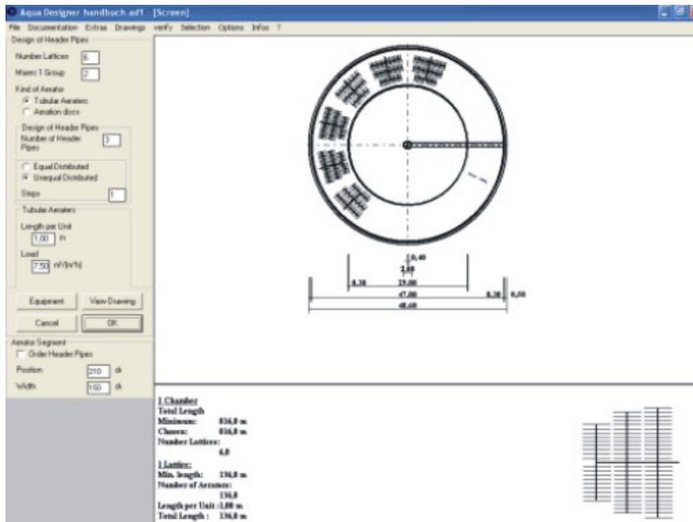
Fig. 141: Combined chamber system, aeration placement
