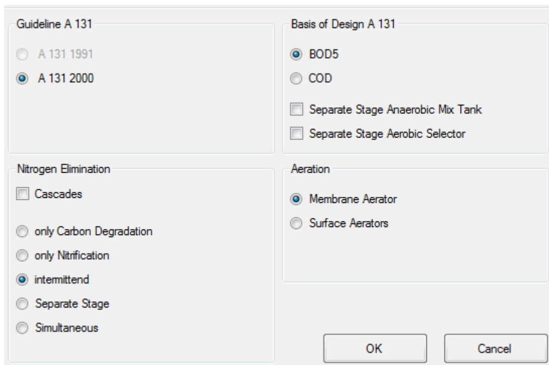
Fig. 158: Options > Process
